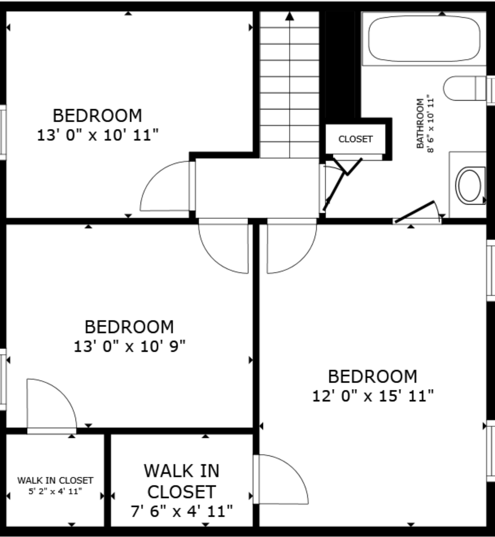
FLOOR 1
